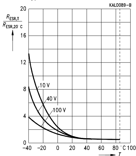
Equivalent series resistance R_{\text{ESR}} at f = 100 \text{ Hz} versus temperature T Typical behavior
