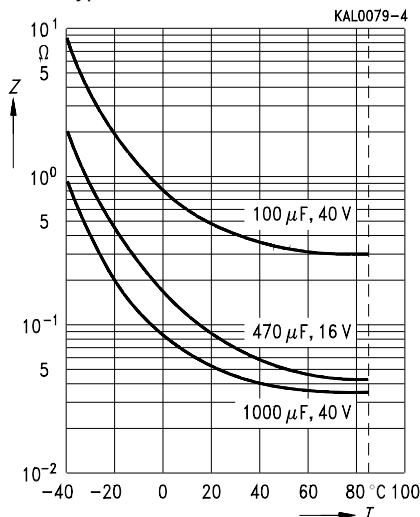
Impedance Z at f = 10 \text{ kHz} versus temperature T Typical behavior
